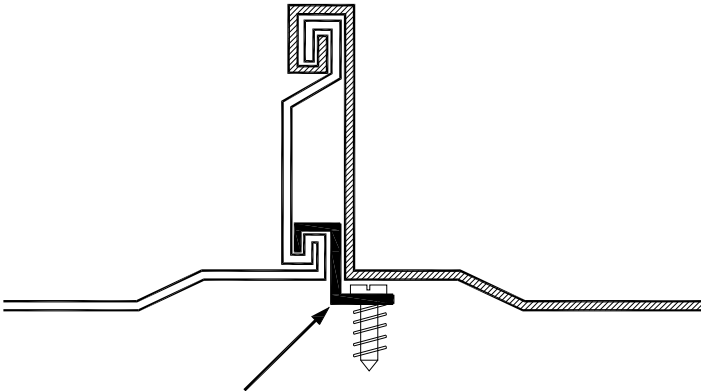
Panel Clip AFTER SEAMING
