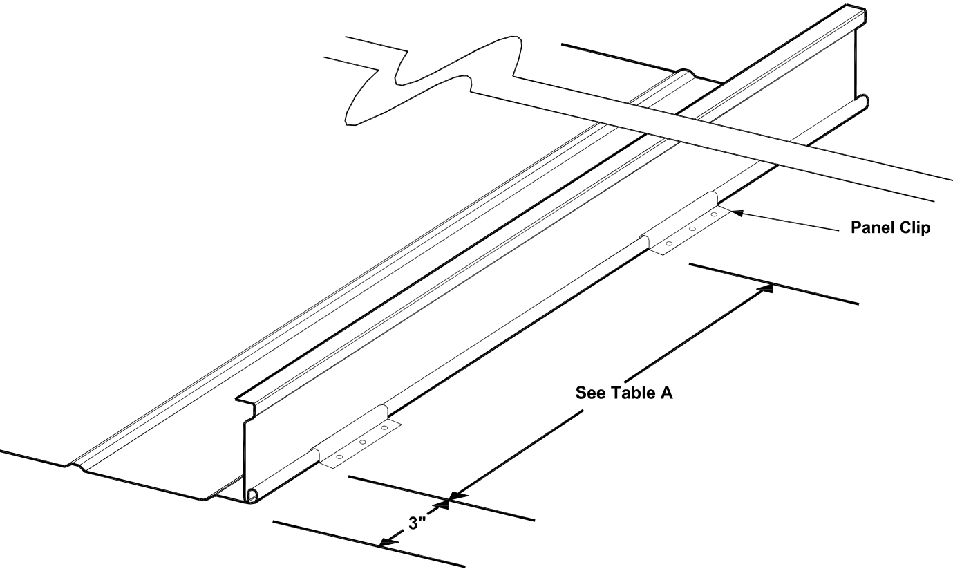
CLIP SPACING DETAIL
