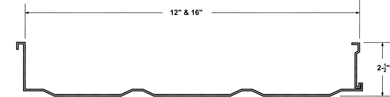
STAND 'N' SEAM STEEL PANEL
