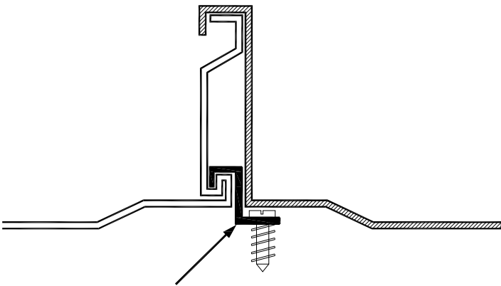
Panel Clip BEFORE SEAMING
